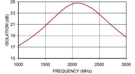
TCP-2-33+ ISOLATION
